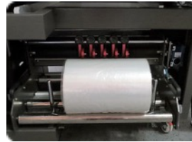
Front Load Film Cradle with Pin Perf Wheels, Saves Space
