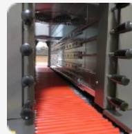
Close Roller Spacing to Transport Unstable Products
